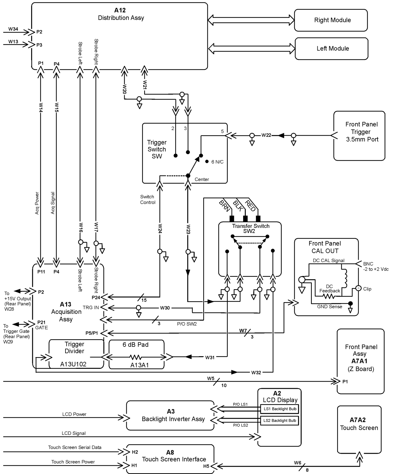
86100B Option 001 Block Diagram (2 of 2)
