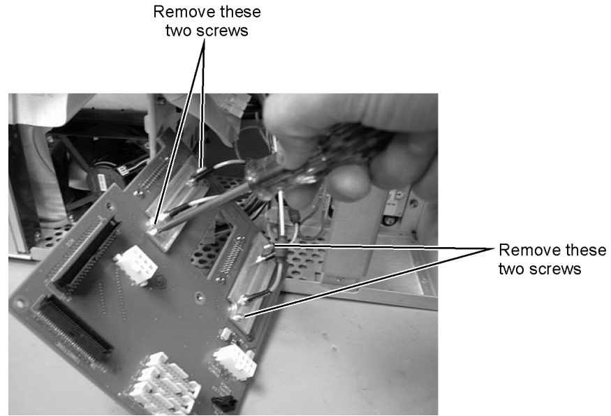
Figure 4-68. Removing the Screws from the A6 Bracket
