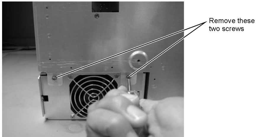
Figure 4-59. Removing the Screws Securing the Power Supply
