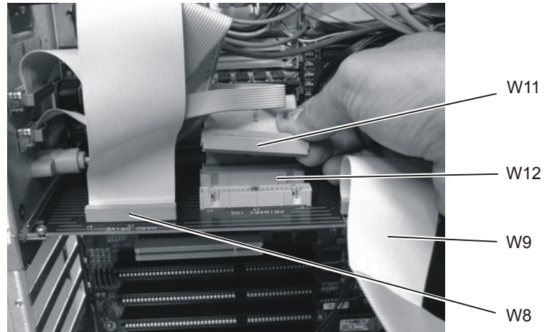
Figure 4-46. W8, W9, W11, and W12 Cables
