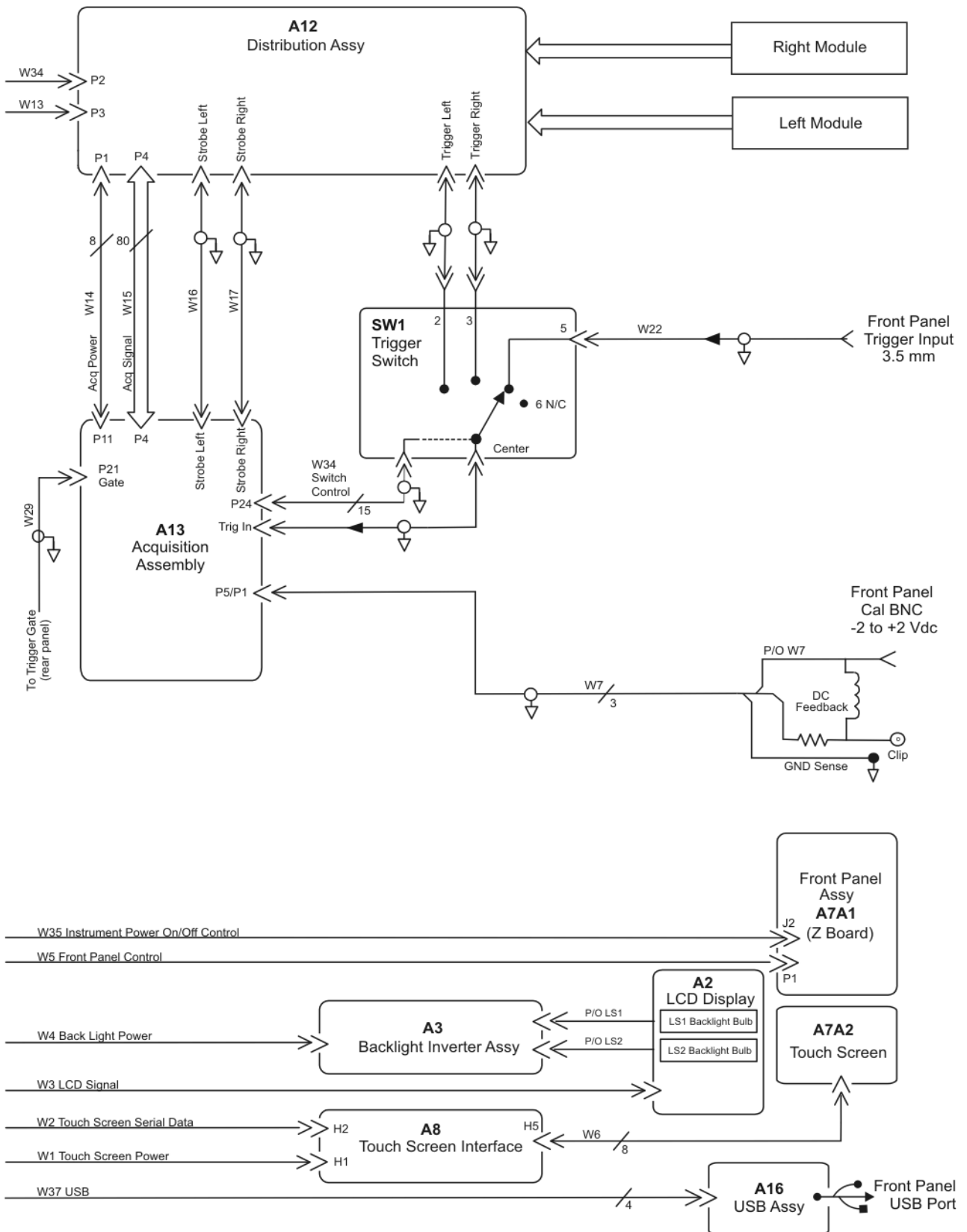
86100C Block Diagram (2 of 2)
