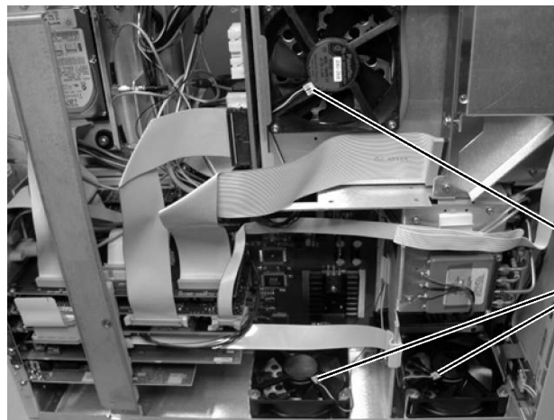
Figure 4-62. Fan Connections
