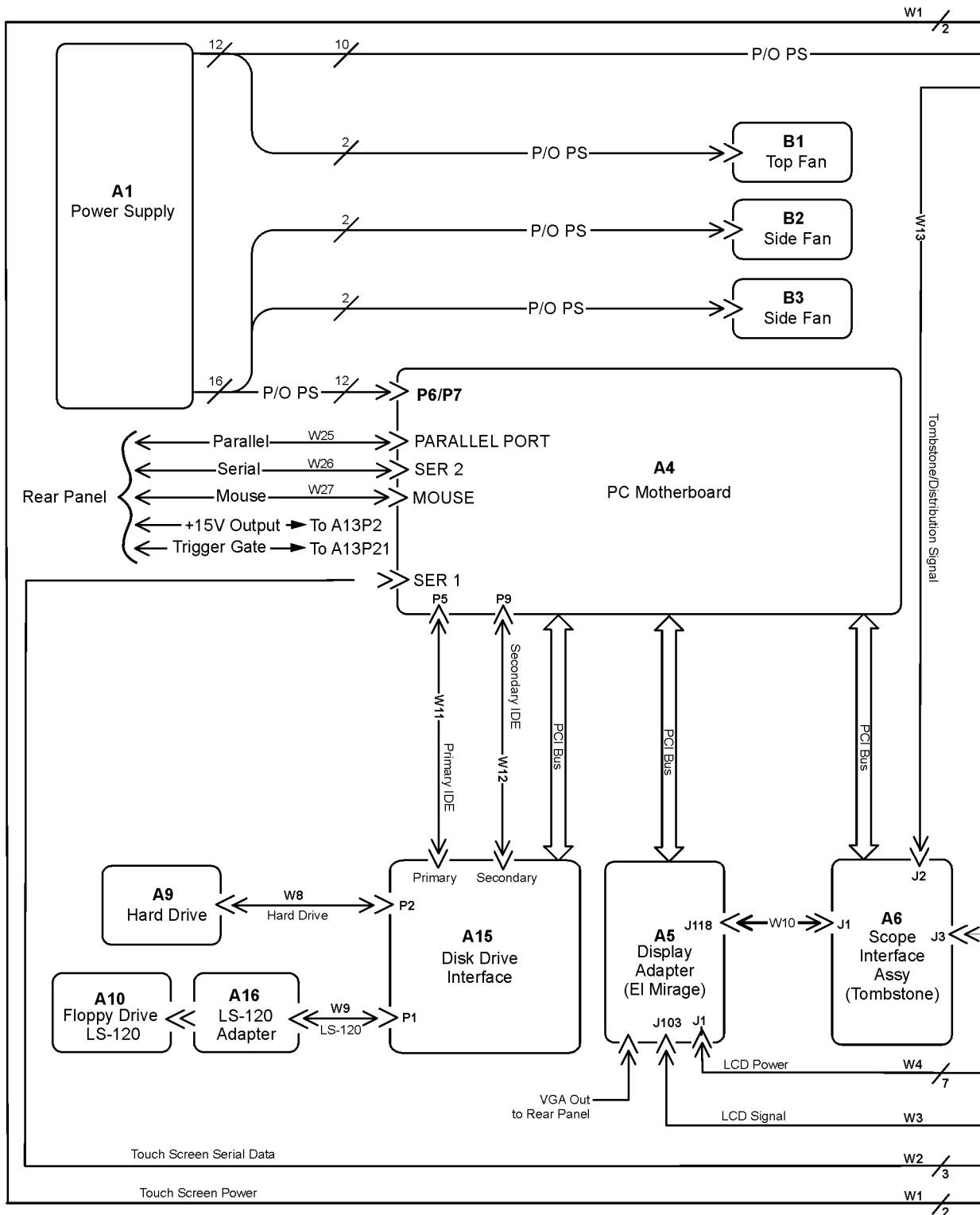
86100A Block Diagram (1 of 2)
