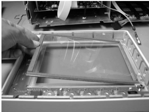
Figure 4-22. Lifting out the Touch Screen
