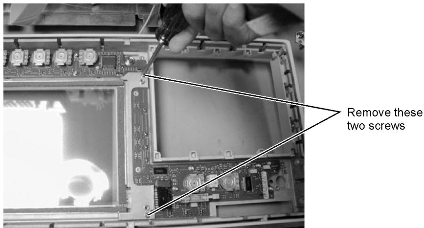
Figure 4-24. Removing the Touch Screen Screws
