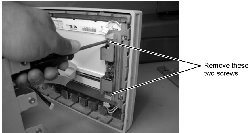
Figure 4-30. Removing the Keyboard Panel Screws
