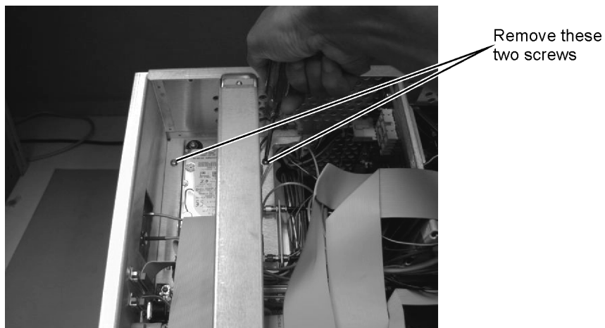
Figure 4-60. Removing the Screws on Top of the Hard Drive
