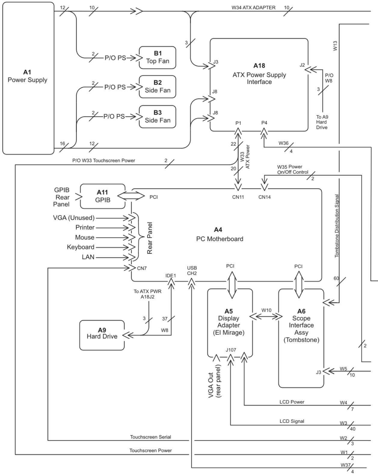
86100C Option 001 Block Diagram (1 of 2)
