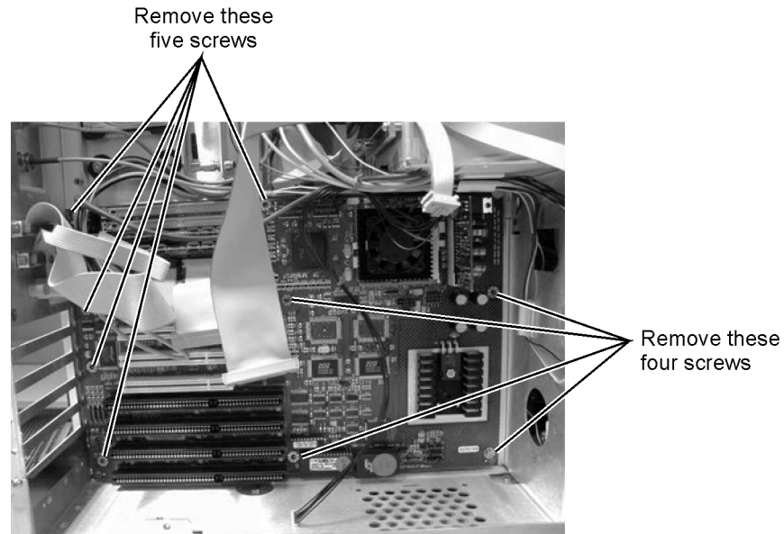
Figure 4-40. Removing the Screws from the Motherboard
