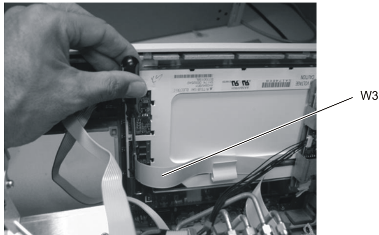
Figure 4-11. Disconnecting the W3 Mylar Flex Cable
