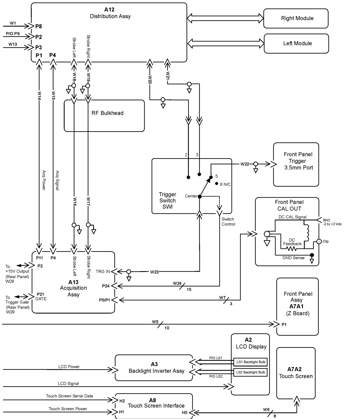
86100A Block Diagram (2 of 2)
