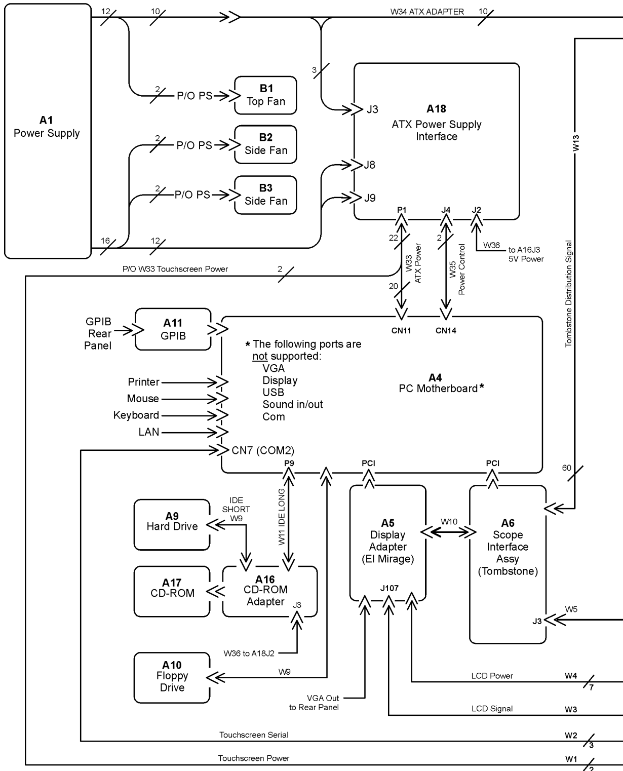
86100B Option 001 Block Diagram (1 of 2)
