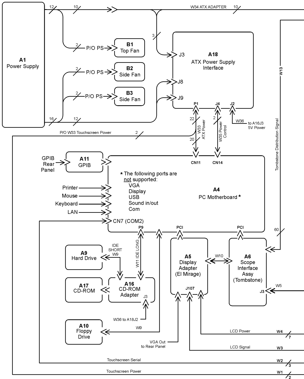
86100B Block Diagram (1 of 2)
