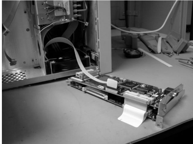
Figure 4-37. Removing the A5 and A6 Boards
