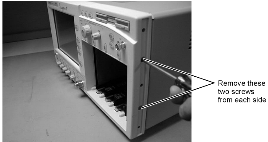
Figure 4-7. Removing the Front Panel Screws
