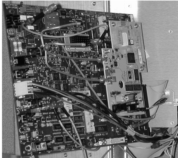
Figure 4-54. 86100C A13 Acquisition Assembly and A14 Counter Assembly
