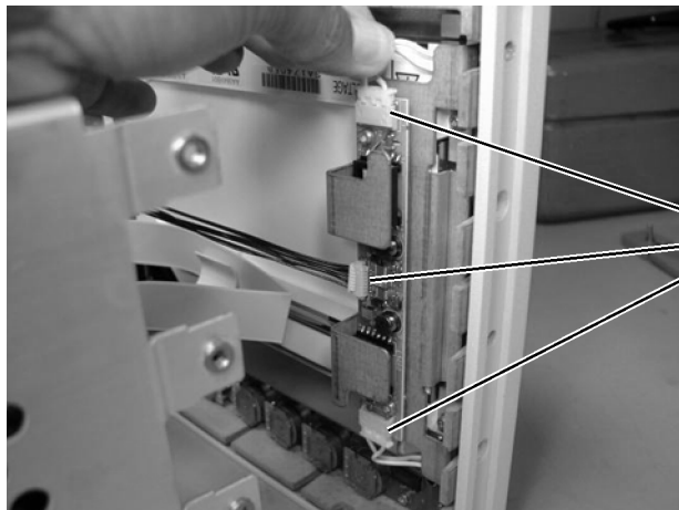
Figure 4-29. Removing the Cables from the Inverter Board
