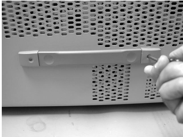
Figure 4-4. Removing the Side Handles
