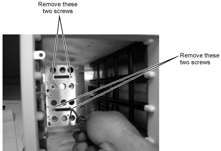
Figure 4-66. Removing Screws from Connectors in Module Drawer
