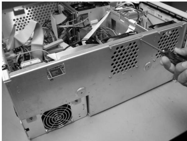
Figure 4-34. Removing the Fan (86100A/B Only)
