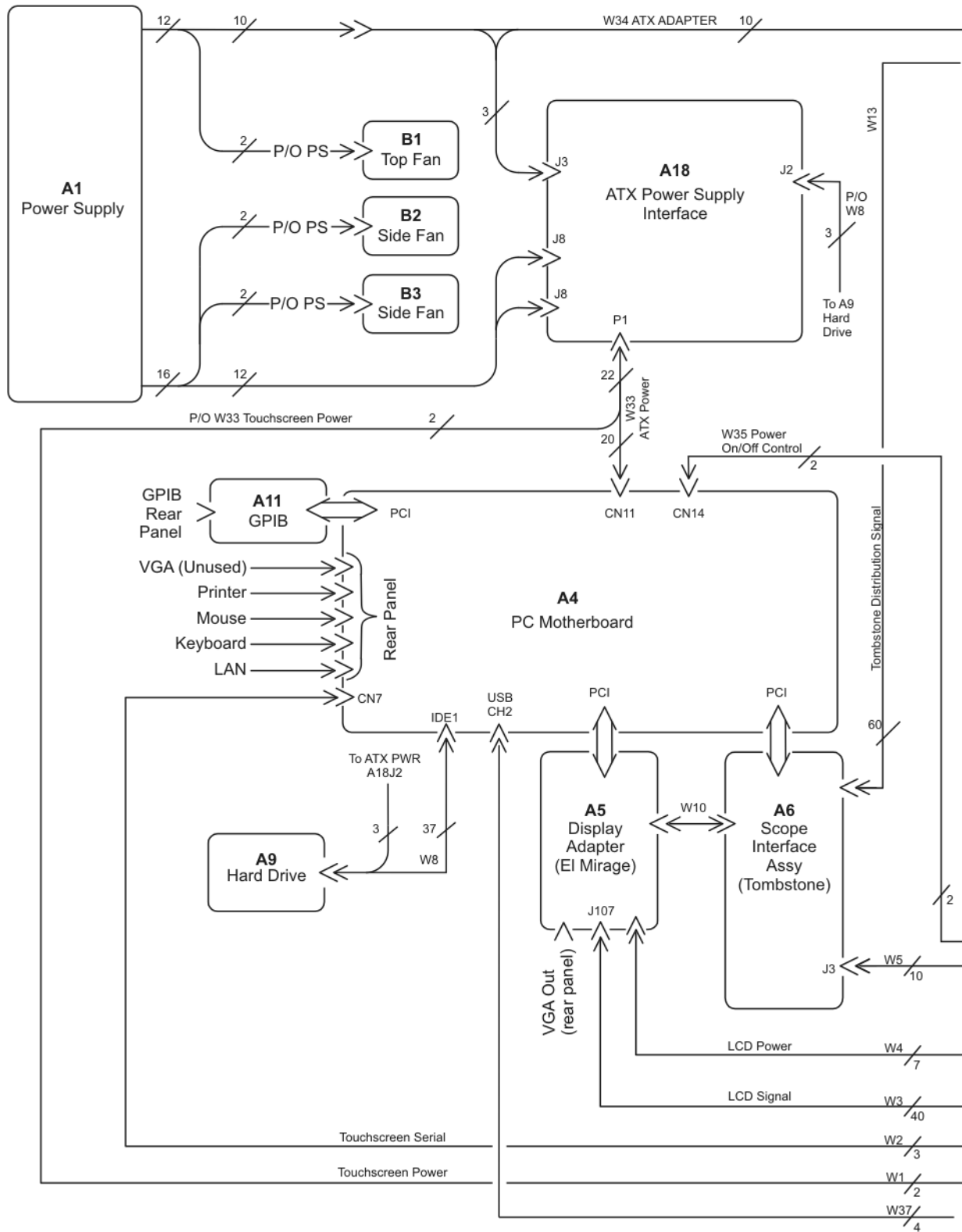
86100C Block Diagram (1 of 2)
