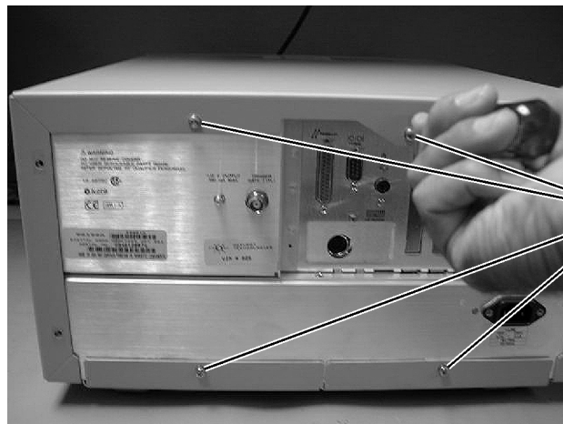
Figure 4-3. Removing Screws from Back of Mainframe
