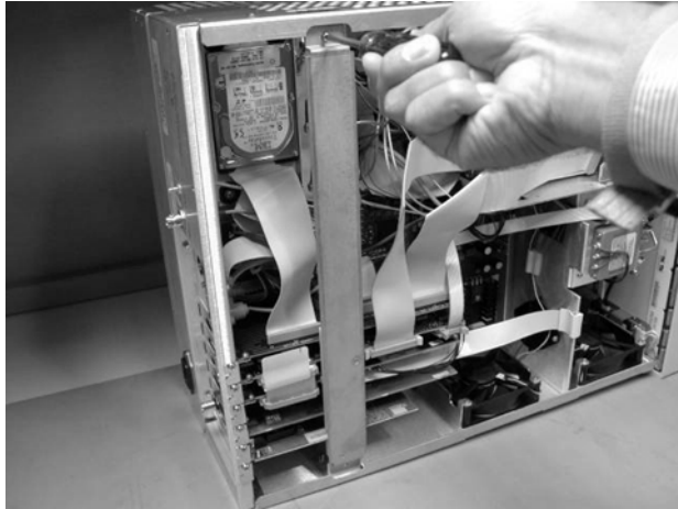
Figure 4-35. Removing the Bar (86100A only)
