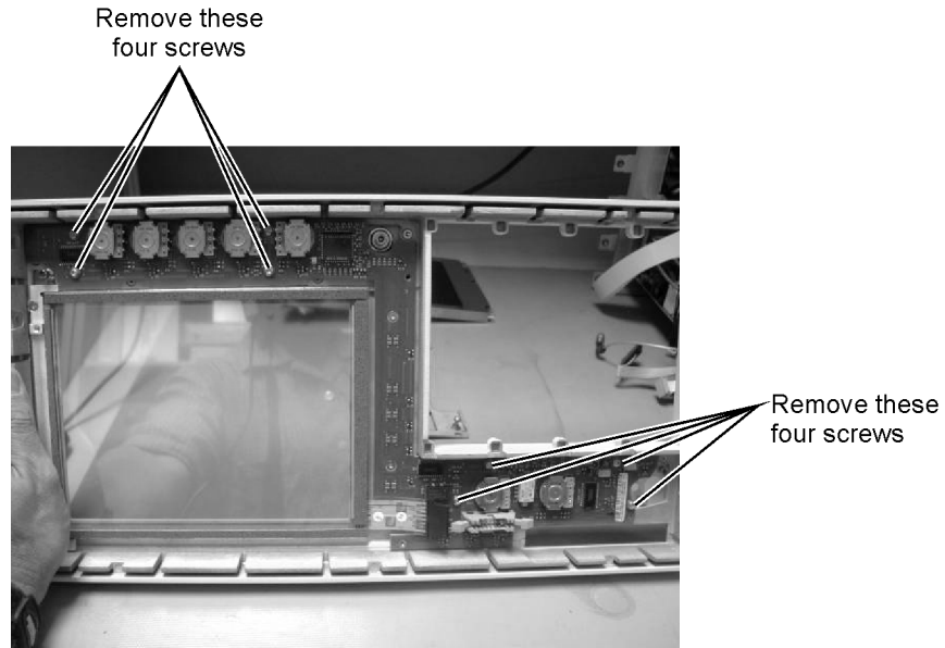
Figure 4-25. Removing the Keyboard Panel Screws
