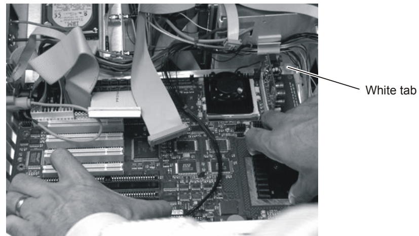
Figure 4-41. Slide the Motherboard Down to Clear the White Tab
