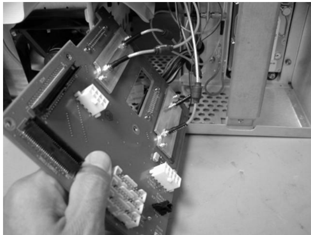
Figure 4-67. Pulling Out the A6 Distribution Assembly Board
