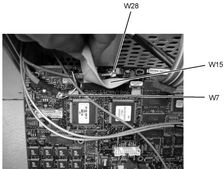
Figure 4-55. W28, W7, and W15 Cables from the A13 Acquisition Board
