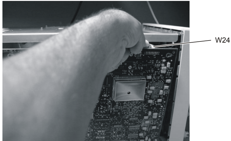
Figure 4-51. Removing the W24 Ribbon Cable from P24 SRC_SEL
