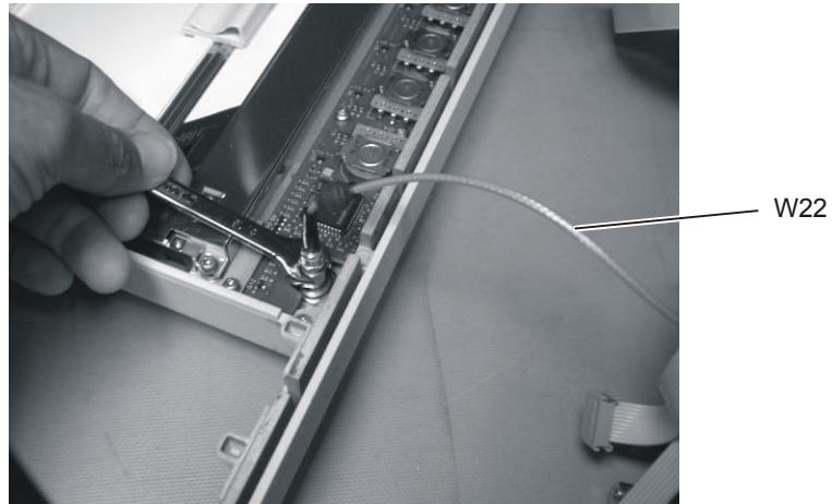
Figure 4-13. Removing the Front Panel Trigger Cable
