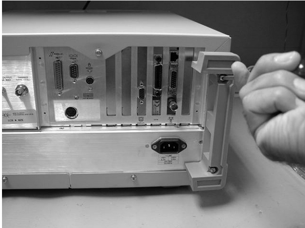
Figure 4-2. Removing the Rubber Feet
