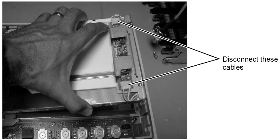
Figure 4-18. Disconnecting the Cables from the A3 Backlight Inverter
