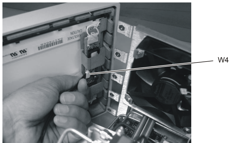
Figure 4-12. Disconnecting the W4 Cable from the A3 Backlight Inverter Board
