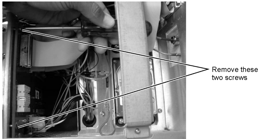
Figure 4-64. Disconnecting Screws from A6 Board
