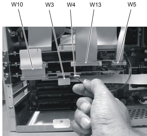
Figure 4-47. W3, W4, W5, W10, and W13 Cables
