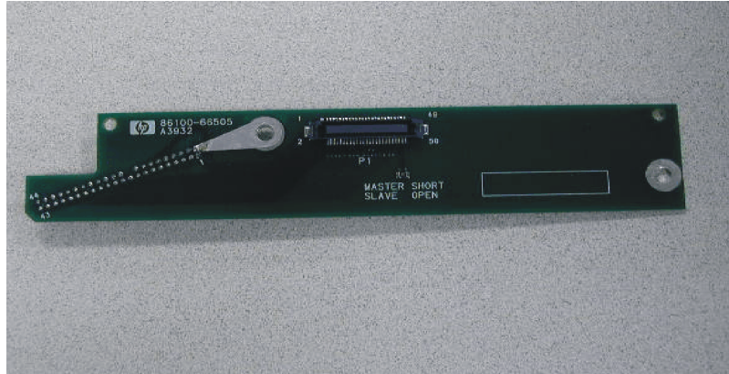
Figure 4-15. A16 LS-120 Board shown with Added Ground Strap
