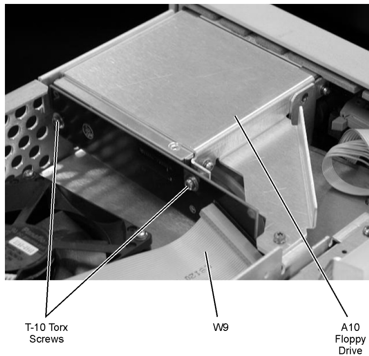
Figure 4-14. LS-120 and A-10 Floppy Drive
