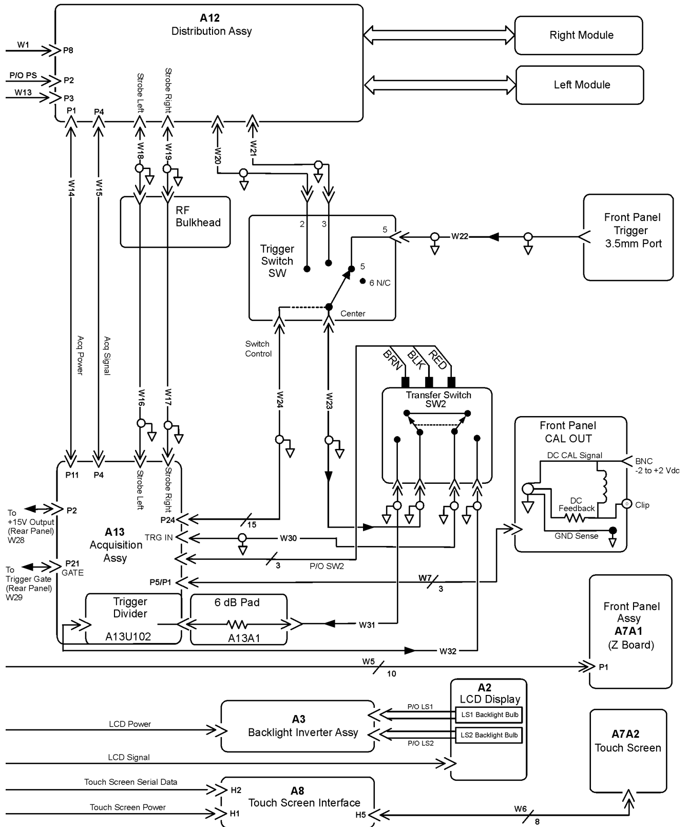
86100A Option 001 Block Diagram (2 of 2)
