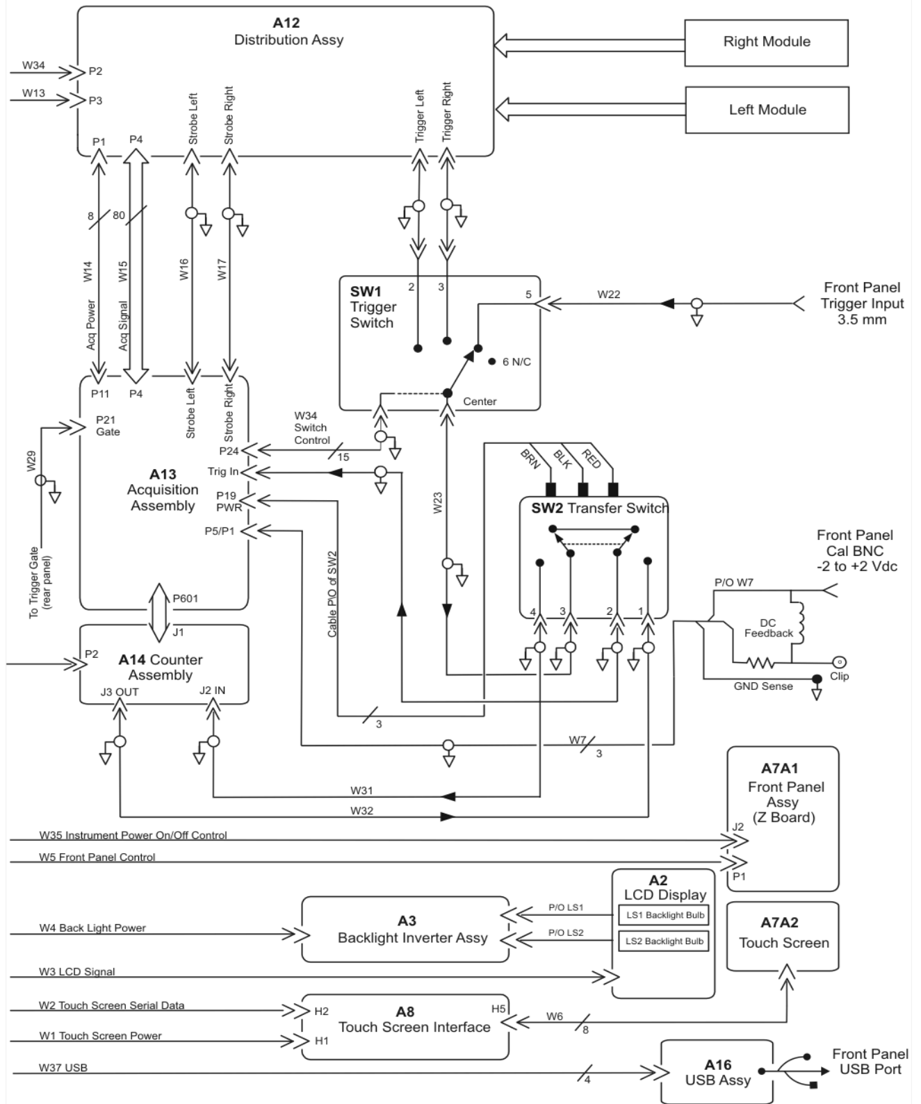
86100C Option 001 Block Diagram (2 of 2)
