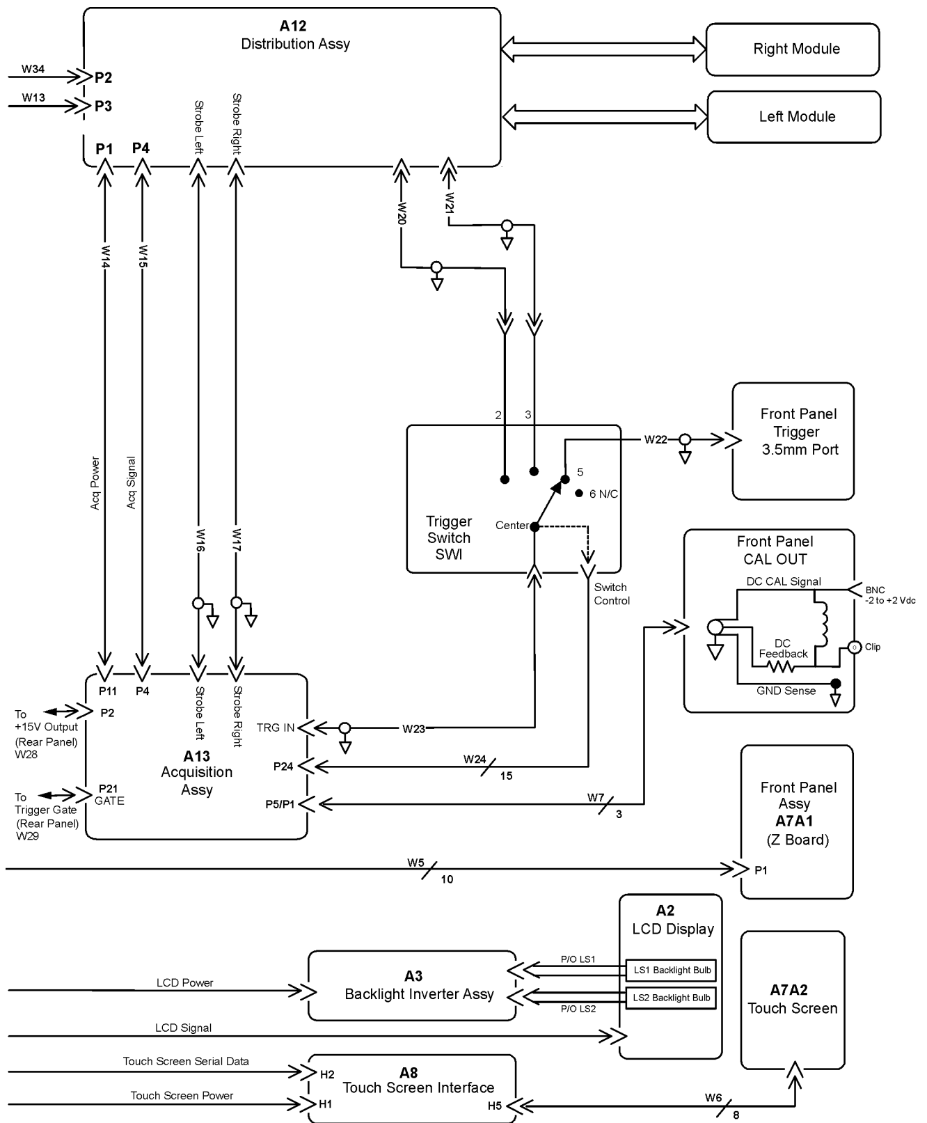
86100B Block Diagram (2 of 2)
