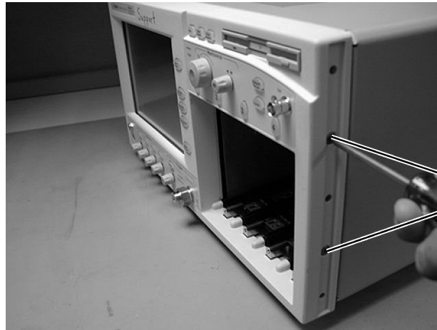
Figure 4-27. Removing the Front Panel Screws
