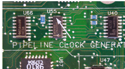
Figure 1-1. U55 location
