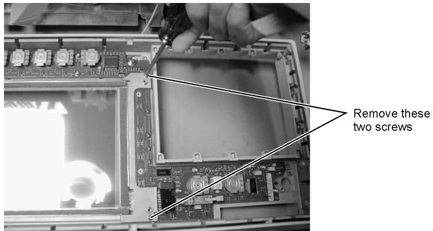
Figure 4-21. Removing the Touch Screen Screws
