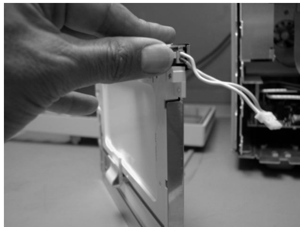
Figure 4-19. Release the Backlight Tab
