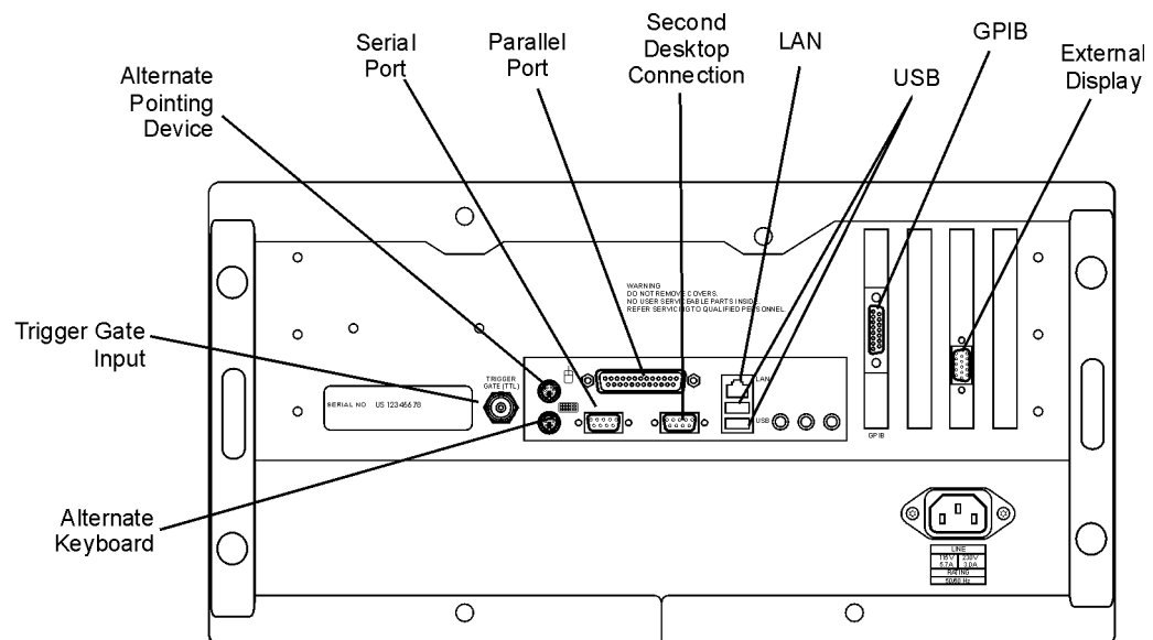
Figure 3-4. Rear Panel Outputs
