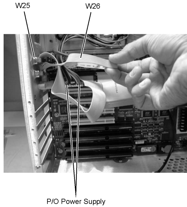
Figure 4-44. W25, W26, and Power Supply Cables
