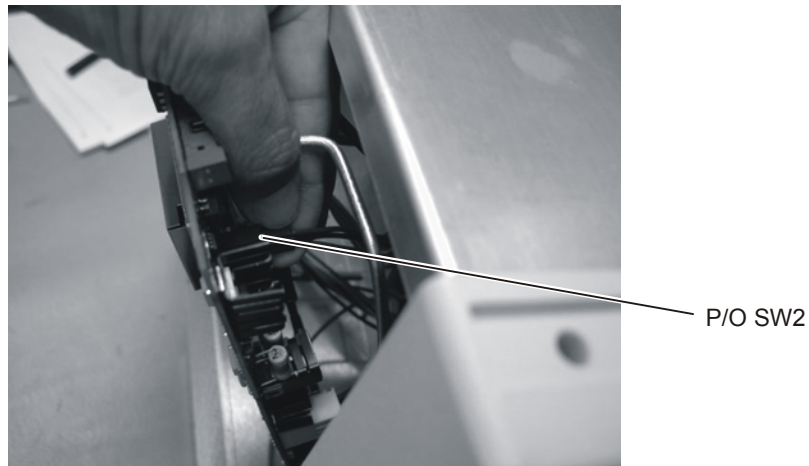
Figure 4-52. Removing the SW2 Cable from P19 Connector
