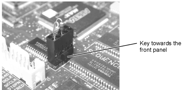
Figure 4-58. Placement of the Jumper on P12
