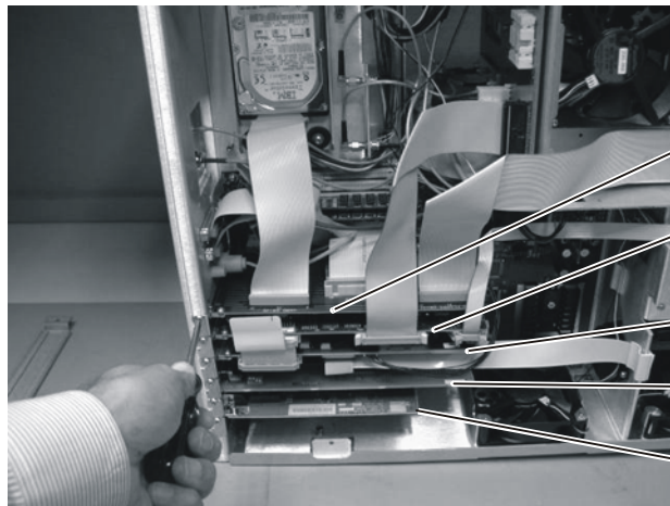
Figure 4-36. Removing the Circuit Boards from the Motherboard
