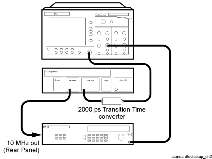
Figure 2-1. Timebase Adjustment Setup
