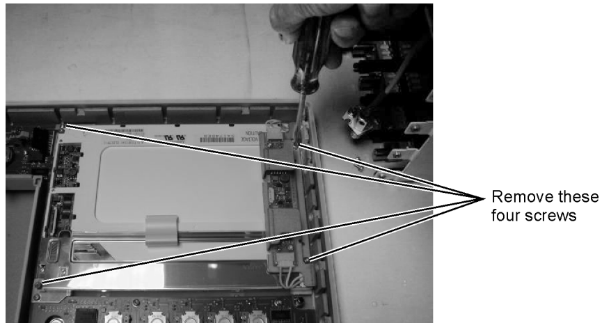
Figure 4-16. Removing the Display Screws
