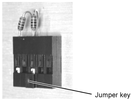
Figure 4-57. Jumper, E2660-01201
