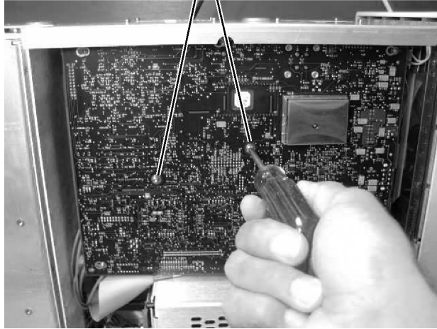
Figure 4-49. Removing the A13 Acquisition Board Screws
