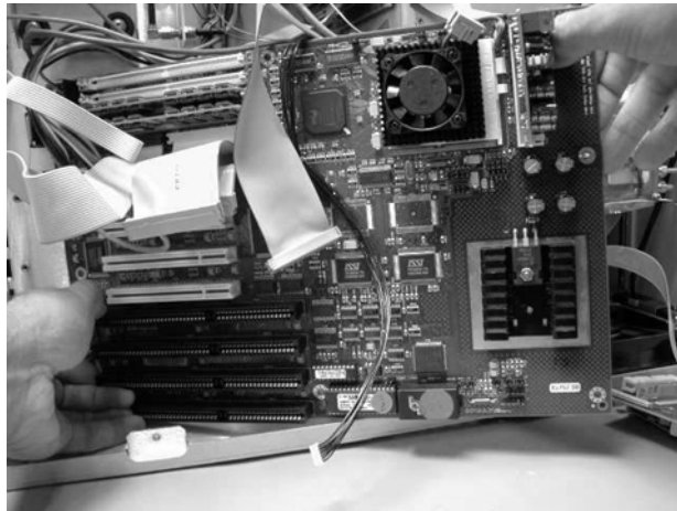
Figure 4-42. Pull the Motherboard out the Right Side
