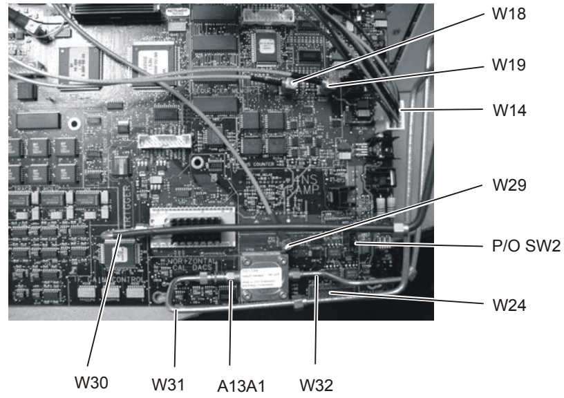
Figure 4-56. Cables from the A13 Acquisition Board (option 001)
